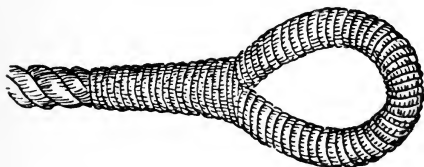
FIG. 94.—Artificial eye (whipped).
